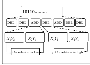
Figure 1: Horizontal Collision Correlation Analysis (HCCA)
