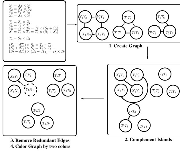
Figure 2: Safe sequence transformation of Edwards curve formula
