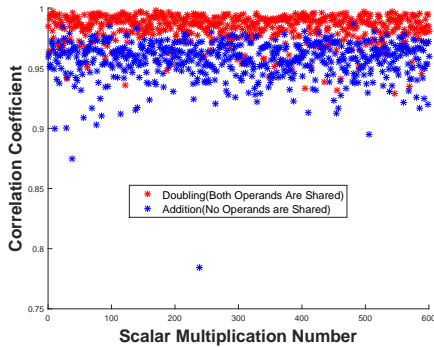
(a) Evaluation of HCCA on Edwards Curve Scalar Multiplier with Correlation
