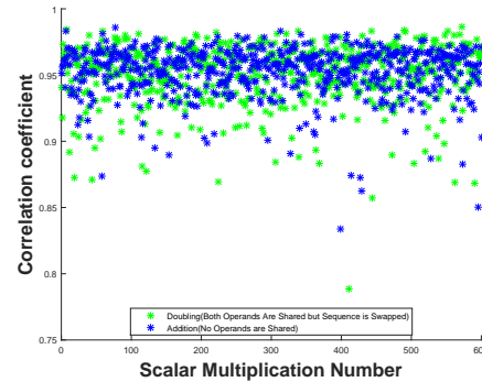
(b) Evaluation of our countermeasure on Edwards Curve Scalar Multiplier with Correlation
