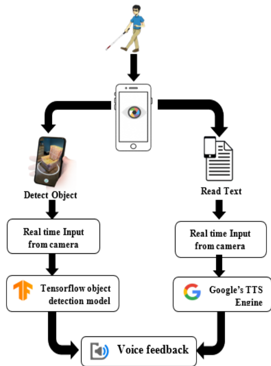
Fig no.1 Flowchart of the proposed system
