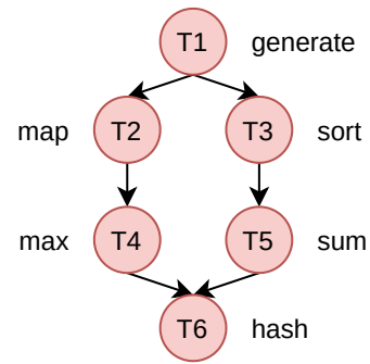
Fig. 2: Task graph for the example application of the case-study.
