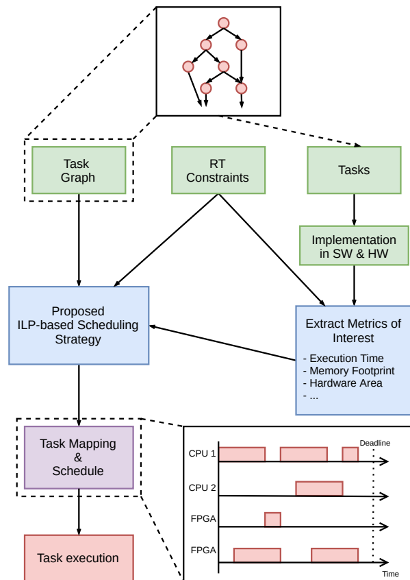
Fig. 1: Overview on our proposed approach.
