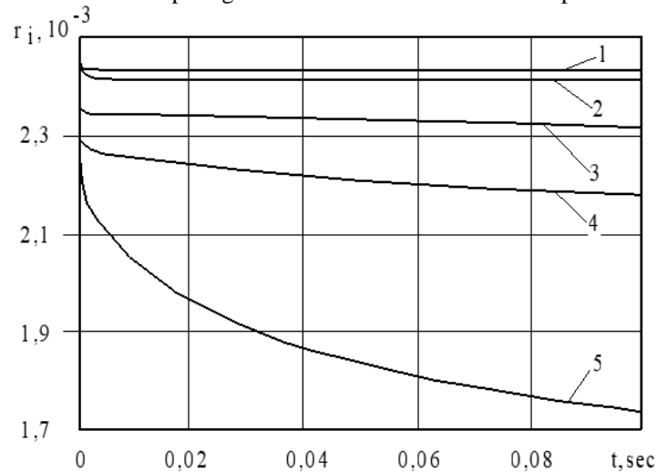
Fig. 2 Change of a mole dose of chlorobenzene at a mass fraction g_3 = 0.01 from composition of mixture and various reference temperatures: 1- 1000 K; 2- 1100 K; 3- 1200 K; 4- 1300 K; 5- 1400 K
