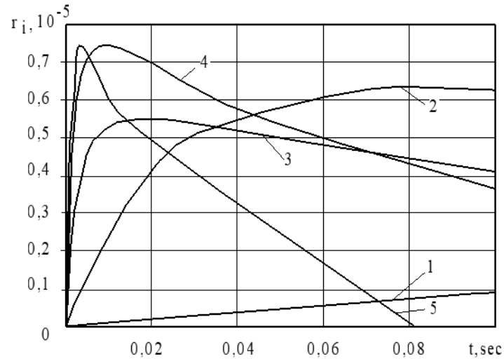
Fig. 3 Change of a mole dose dichlorobenzene at a mass fraction of chlorobenzene g = 0.0001 from composition of mixture and various reference temperatures: 1- 1000 K; 2- 1100 K; 3- 1200 K; 4- 1300 K; 5- 1400 K
