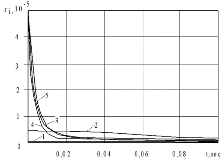
Fig. 5 Change of a mole dole atomic hydrogen H at a mass fraction of chlorobenzene g = 0.0001 from composition of mixture and various reference temperatures: 1- 1000 K; 2- 1100 K; 3- 1200 K; 4- 1300 K; 5- 1400 K
