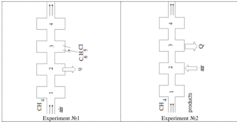
Fig. 1 The scheme of a mathematical model for carrying out a numerical experiment
