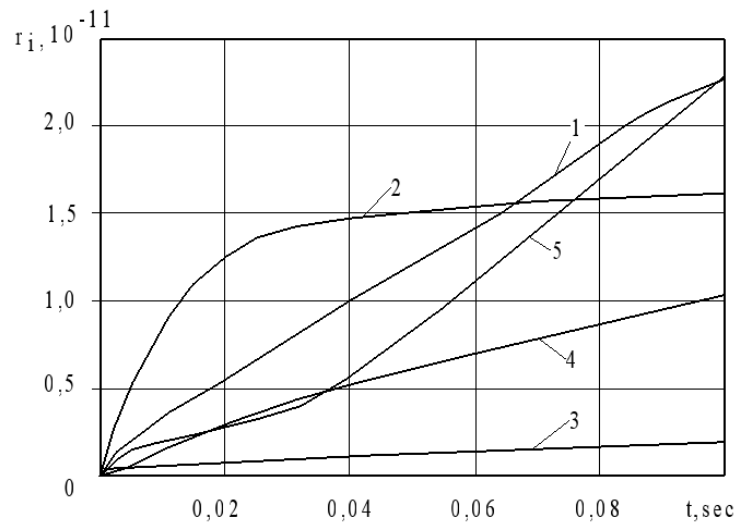
Fig. 4 Change of a mole dose chloromethane CH_3Cl at a mass fraction of chlorobenzene g = 0.0001 from composition of mixture and various reference temperatures: 1- 1000 K; 2- 1100 K; 3- 1200 K; 4- 1300 K; 5- 1400 K
