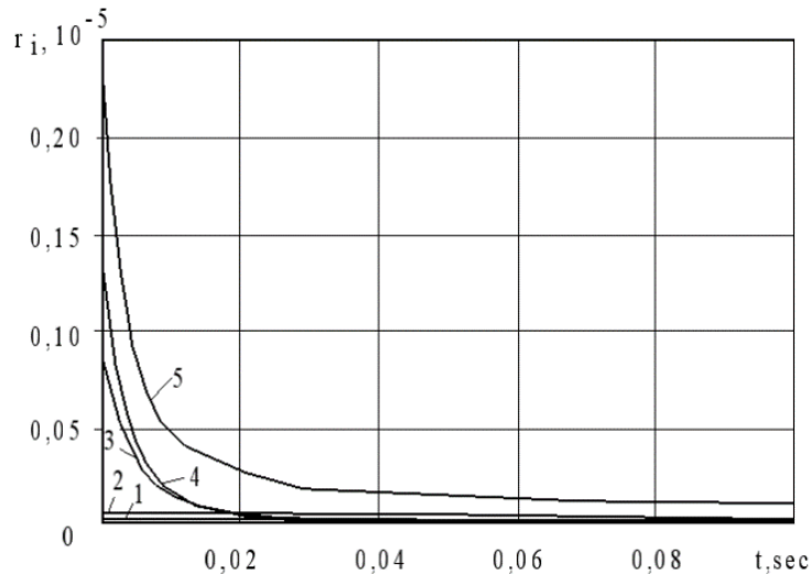
Fig. 6 Change of a mole dole OH at a mass fraction of chlorobenzene g = 0.0001 from composition of mixture and various reference temperatures: 1- 1000 K; 2- 1100 K; 3- 1200 K; 4- 1300 K; 5- 1400 K
